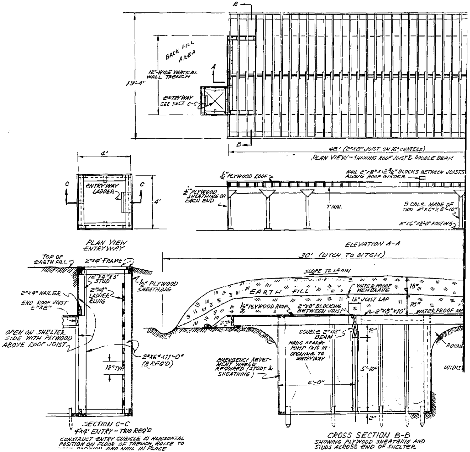
Fig. A-8.1. Trench Walls, Underground Shelter.
